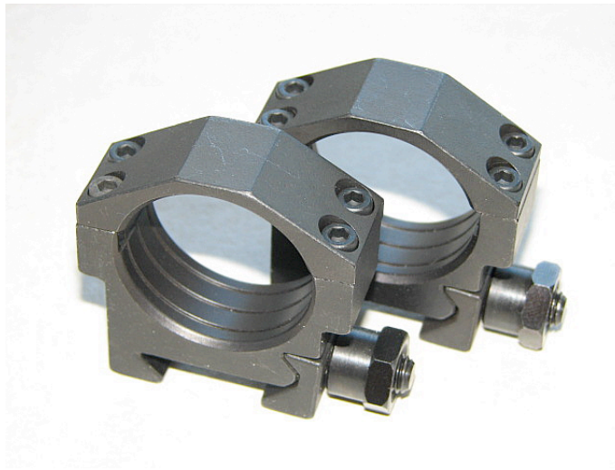
30mm HD Low (0.25" High) Rings, P/N 7002 Depicted
